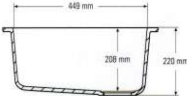
Side cross-section
