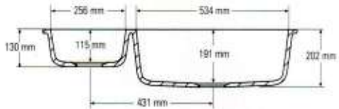
Front cross-section
