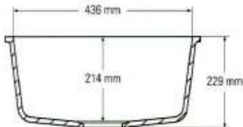
Side cross-section
