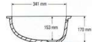
Side cross-section
