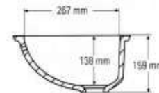
Side cross-section
