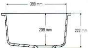
Side cross-section
