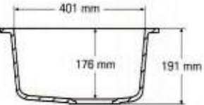
Side cross-section
