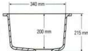
Side cross-section
