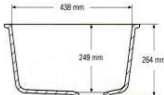
Side cross-section
