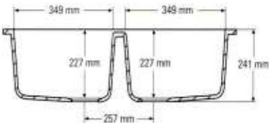
Front cross-section
