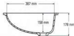
Side cross-section
