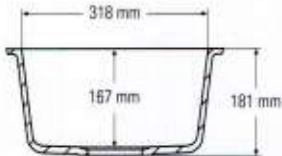
Side cross-section
